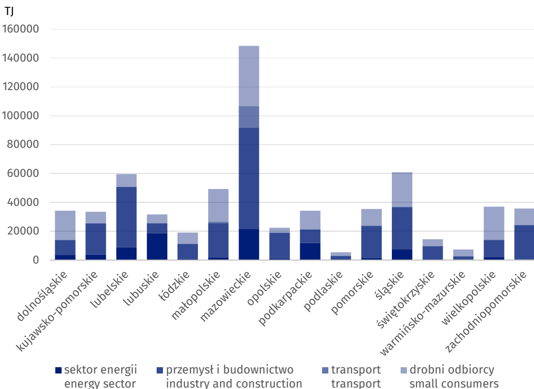
Chart 2. Consumption of natural gas in 2017
