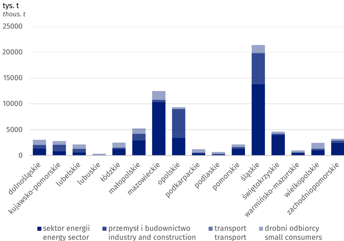
Chart 1. Consumption of hard coal in 2017
