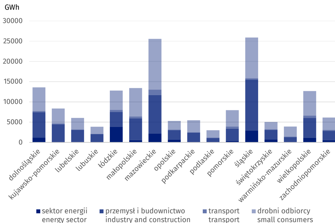
Chart 4. Consumption of electricity in 2017
