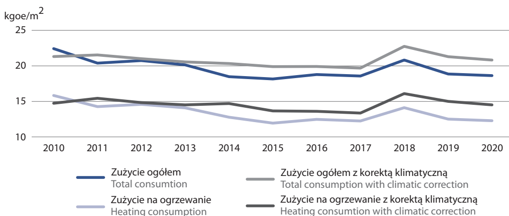
Chart 17. Energy consumption in households per m 2
