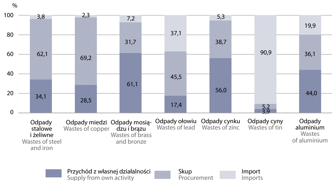
Chart 18. Supply of metallic wastes suitable for recycling in production units in 2022
