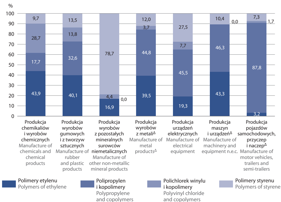
Chart 9. Structure of consumption of selected plastics by selected NACE divisions of manufacturing in 2020
