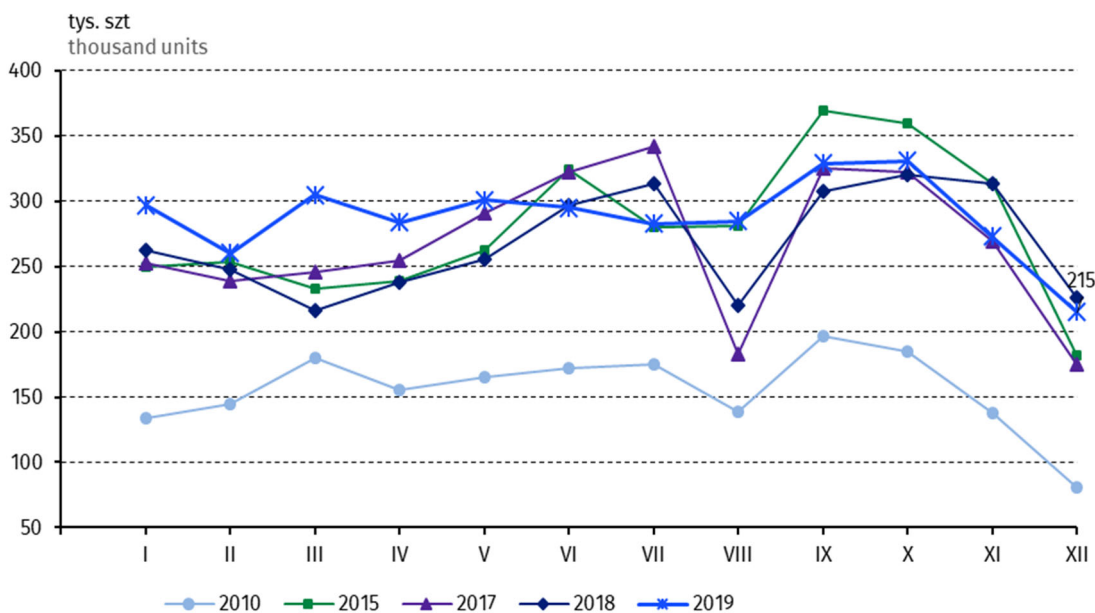
Chart 12. Production of refrigerators and freezers b
