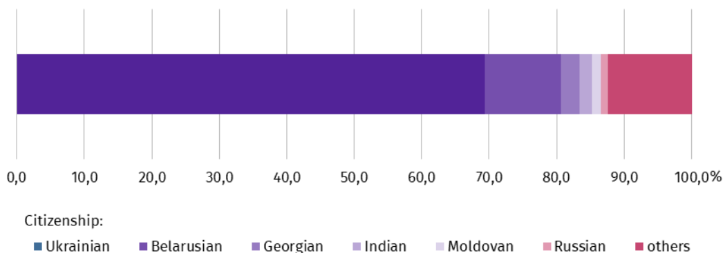
Chart 2. Structure of foreigners performing work by citizenship in 2023 As at 31 July
