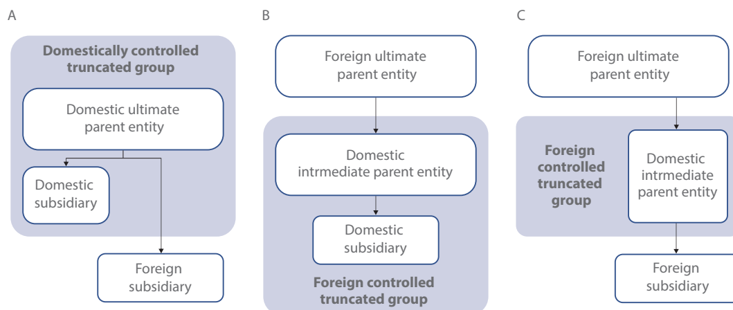
Figure 1. Examples of structures of truncated groups
