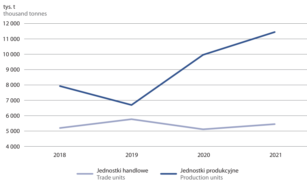
Chart 17. Supply of steel and iron wastes suitable for recycling in production and trade units in 2018–2021
