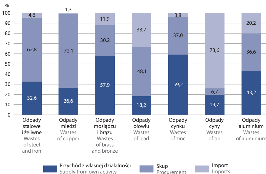
Chart 13. Structure of supply of metallic wastes suitable for recycling in production units in 2021
