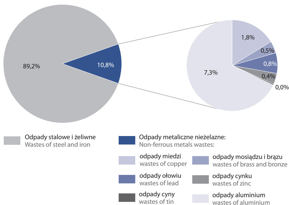
Chart 25. Structure of supply of metallic wastes suitable for recycling in production units in 2021
