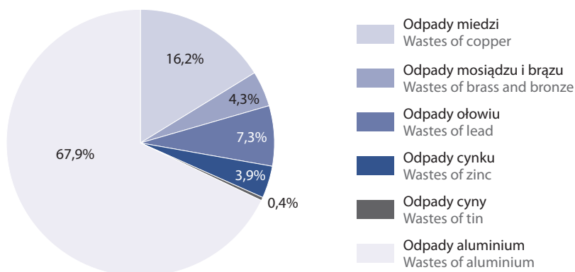
Chart 26. Structure of supply of non-ferrous metals wastes suitable for recycling in production units in 2021
